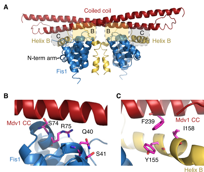
FIGURE 3. Two binding interfaces on surface of Mdv1 coiled coil. A , ribbon representation of the Mdv1-Fis1 structure, with shaded regions indicating interactions mediated by the long coiled coil. The tan shading highlights the interface shown in B ; the gray shading highlights the interface shown in C . Because of the 2-fold symmetry of the dimer, the bottom surface of the coiled coil makes four contacts. B , interaction of the Mdv1 coiled-coil surface with residues on the top surface of Fis1. Residues mutated in this study are indicated (stick representation). C , interaction of the Mdv1 coiled-coil surface with the Mdv1 \alpha B helix. Residues mutated in this study are indicated.
