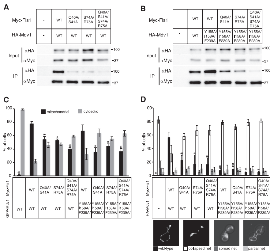
FIGURE 4. Functional analysis of Mdv1-Fis1 interfaces. A , co-immunoprecipitation of HA-Mdv1 by Myc-Fis1 variants. The mutant Fis1 constructs contain the indicated mutations. In the lower panel , anti-Myc immunoprecipitates were analyzed by Western blotting with anti-HA and anti-Myc antibodies. B , co-immunoprecipitation of HA-Mdv1 Y155A/I158A/F239A by Myc-Fis1 variants. The mutant combinations are indicated. In the lower panel , anti-Myc immunoprecipitates were analyzed by Western blotting with anti-HA and anti-Myc antibodies. C , subcellular localization of GFP-Mdv1 in yeast mutants. The localization of GFP-Mdv1 was scored as “cytosolic” when a diffuse green signal was present in the cytosol and as “mitochondrial” when green puncta were localized to mitochondria. The mutant combinations are indicated. *, p \leq 0.001 (unpaired t test) compared with wild-type Mdv1-Fis1. The Y155A/I158A/F239A mutant was not statistically different from the wild type. D , mitochondrial morphology in mutant yeast. Yeast cells were scored into four categories as described previously (17). Representative images of the four categories are shown. The mutant combinations are indicated. *, p \leq 0.01 compared with wild-type Mdv1-Fis1. In C and D , the error bars indicate S.D. from three independent experiments. In each experiment, 100 live yeast cells were scored.
